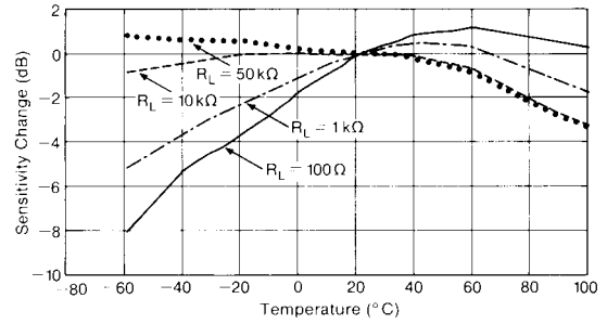
Figure 5. Typical output response with temperature. ( P_{in} \leq 20 \text{ dBm} )
